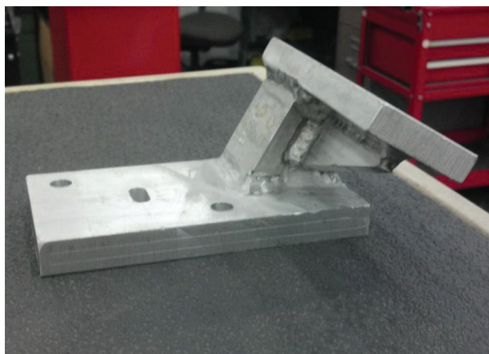
Weldment
