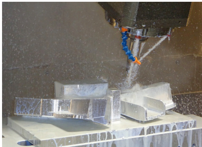
5-Axis Machined Aircraft Structural Bracket
